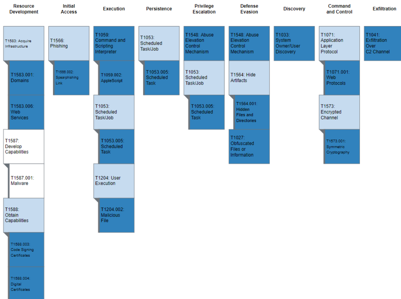
Figure 2: MITRE ATT&CK enterprise techniques used by Applejeus
